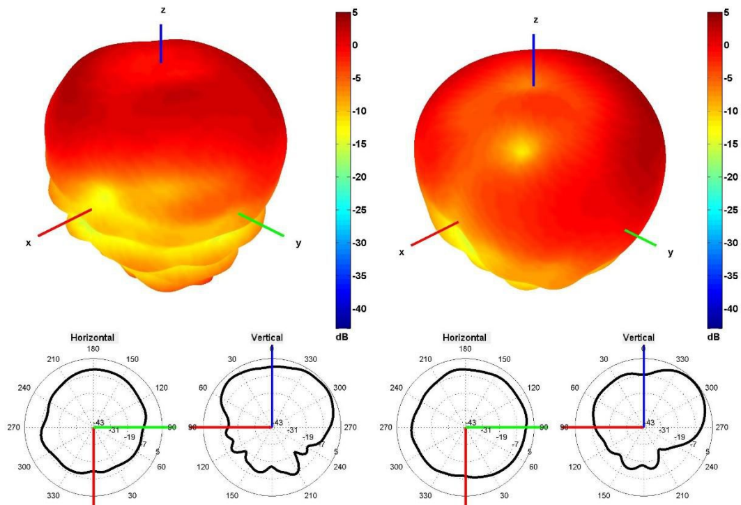
1950 and 2070 MHz Radiation pattern
