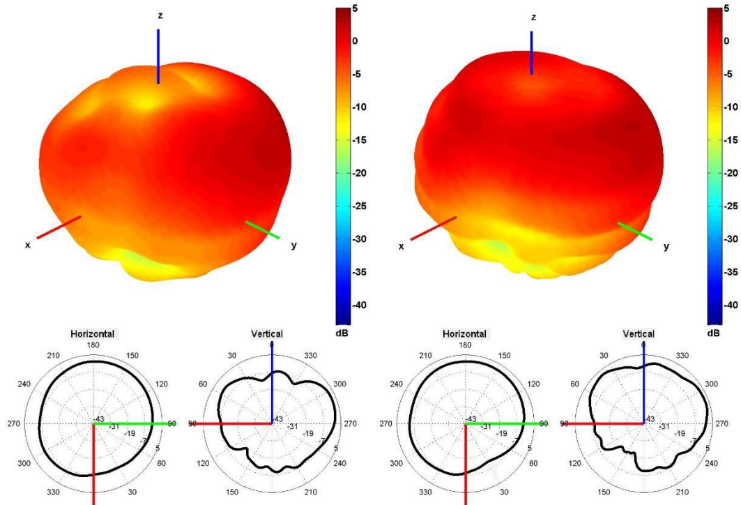
1750 and 1830 MHz Radiation pattern
